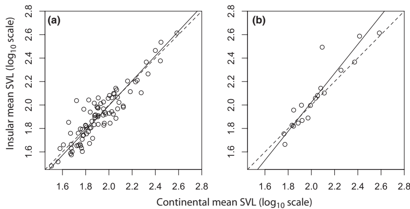
Figure 2 Standardized major axis regression of mean body size [ \log_{10} -transformed snout-vent length (SVL) in mm] on islands versus continents for species in lizard genera (a) and families (b). The dashed line has a slope of 1 and an intercept of 0. The solid line represents the standardized major axis regression slope estimate.
