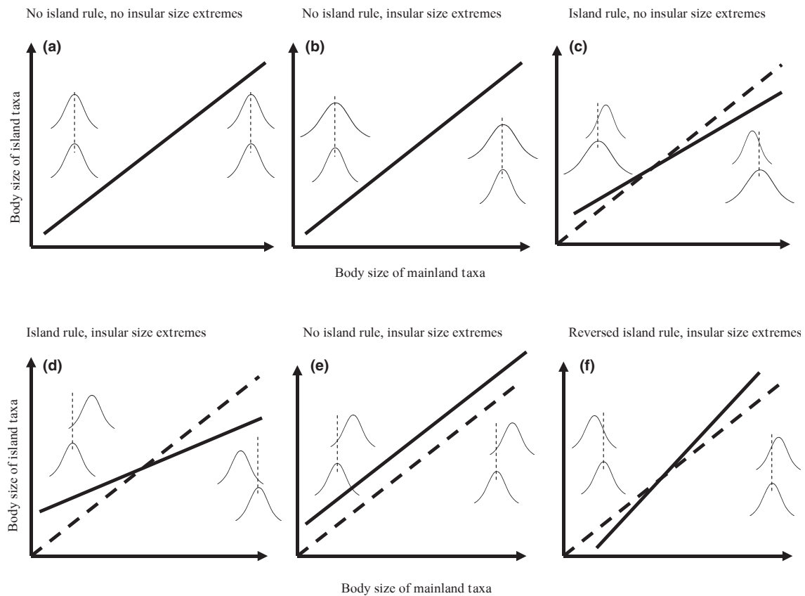
Figure 1 Schemes showing possible ways in which patterns of body size on islands and mainland within taxa (size extremes or average sizes) can combine to produce patterns of body size across taxa (slope <1 , slope =1 , slope >1 ). x-axis, mainland body size; y-axis, island body size; dashed line, a line with an intercept of 0 and a slope of 1; solid line, slope returned by standardized major axis regression (can mask the dashed line). The body size frequency distributions depict insular (top) and mainland members of a clade (bottom). The mainland mean size is indicated by the vertical, dashed line. (a) The null distribution. No insular size extremes, no island rule (slope of 1, similar insular and mainland size ranges). (b) There are size extremes because island taxa have wider size distributions, but no island rule because mean sizes are similar (slope of 1). (c) The island rule holds (small animals evolve larger size and large ones dwarf, slope <1 ), but no size extremes because island taxa have narrower size distributions. (d) The island rule holds (slope <1 ), and insular clades are of extreme size – members of large-bodied clades are smallest in their clade and members of small-bodied clades are the largest in their clade. (e) Island members are proportionally always larger than mainland ones, hence there is one type of size extreme, but no island rule (no dwarfing of large animals, slope =1 ). (f) There are size extremes, but in the opposite direction than predicted under the island rule. Small-sized insular animals are extremely small, large ones are extremely large (slope >1 ).
