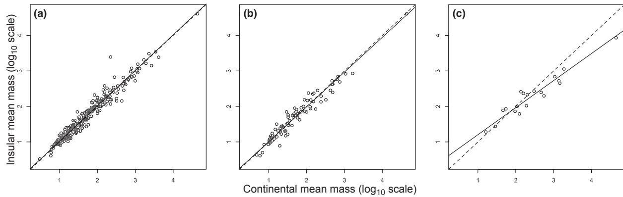
Figure 3 Standardized major axis regression of mean body size ( \log_{10} -transformed mass, in g) on islands versus continents for species in bird genera (a), families (b) and orders (c). The dashed line has a slope of 1 and an intercept of 0. The solid line represents the standardized major axis regression slope estimate.
