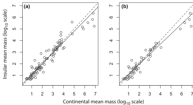
Figure 5 Standardized major axis regression of mean body size ( \log_{10} -transformed mass, in g) on islands versus continents within (a) mammalian sister clades and (b) a subset of the data in (a): only sister species [only clades in (a) where both mainland and insular sample sizes are 1]. The dashed line has a slope of 1 and an intercept of 0. The solid line represents the standardized major axis regression slope estimate.
