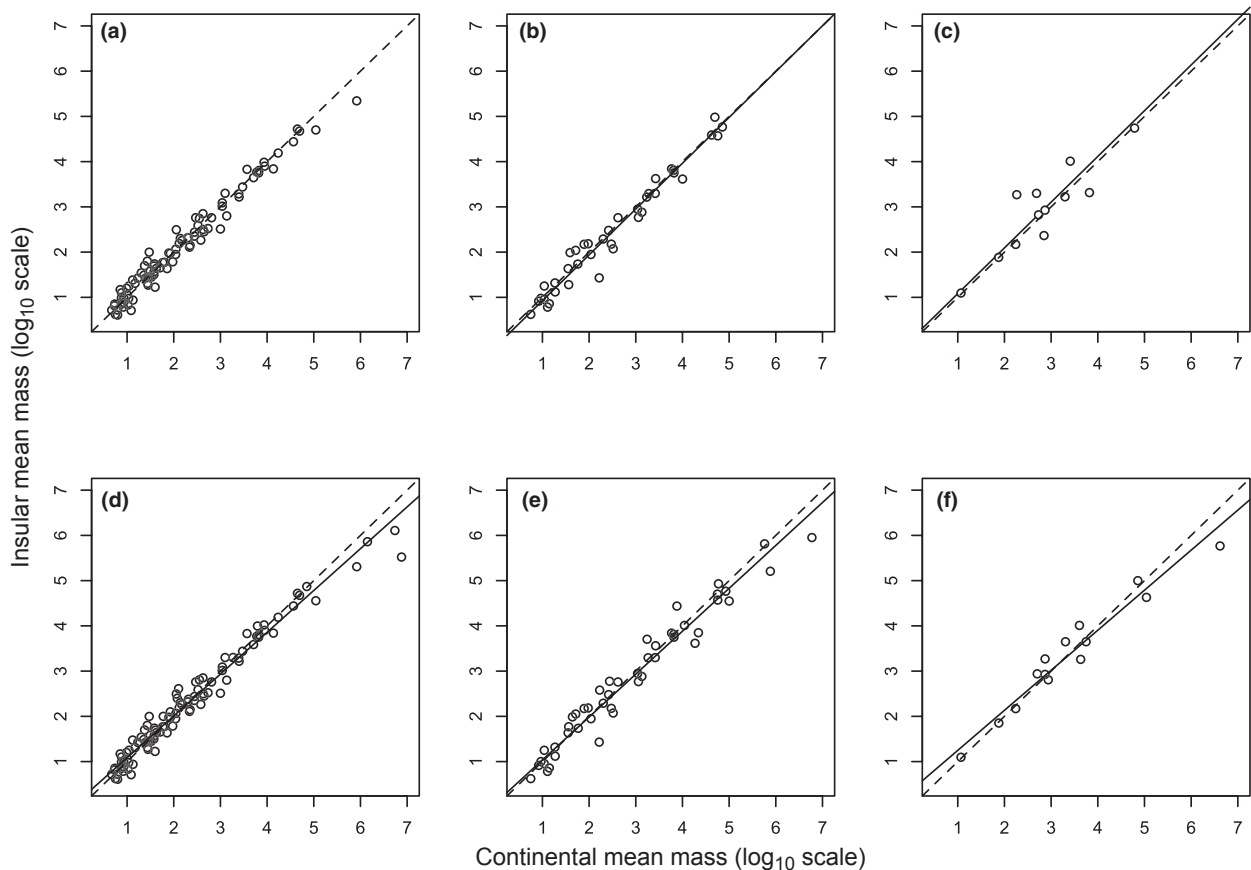
Figure 4 Standardized major axis regression of mean body size ( \log_{10} -transformed mass, in g) on islands versus continents for species in mammalian genera (a, d), families (b, e) and orders (c, f). Plots (a)–(c) are for extant taxa only and (d)–(f) include extinct taxa (see Materials and Methods). The dashed line has a slope of 1 and an intercept of 0. The solid line represents the standardized major axis regression slope estimate.
