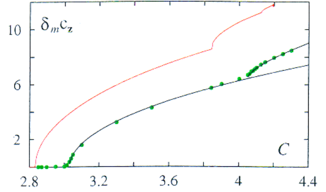
Fig. 18. Domain of period-doubling oscillations in the Rössler medium supporting a spiral wave. The upper red curve is for the Rössler ordinary differential equation.
