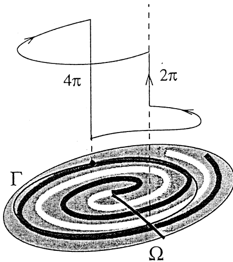
Fig. 11. Advance of the oscillation phase along contour \Gamma in the period-2 medium. The local angle variable field \varphi(\mathbf{r}, t_0) of a spiral wave is schematically shown by gray shades.
