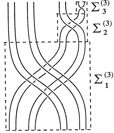
Fig. 17. Braid B_8 constructed for the period-8 orbit.
