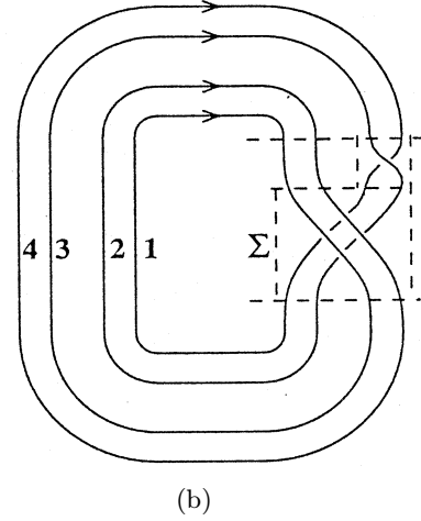
Fig. 14. Projection of the period-4 orbit of the Willamowski-Rössler system on (a) the (c_x, c_y) plane and (b) the corresponding closed braid \overline{B}_4 .
