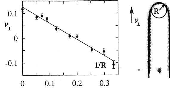
Fig. 25. Dependence of the domain propagation velocity, v_{\perp} , versus the curvature, 1/R , of the tip for C = 4.30 . A typical finger-shaped \Omega_2 domain is shown in the right panel.
