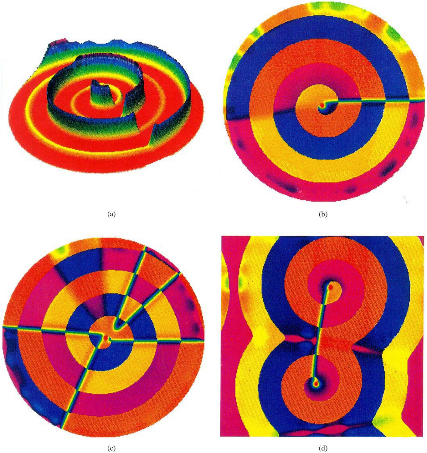
Fig. 12. Synchronization defect lines in Rössler media with period-4 dynamics for C = 4.30 : (a) instantaneous c_z(\mathbf{r}) concentration profile of a single spiral wave is shown both by elevation and color; (b) synchronization defects in the medium shown in panel (a) are visualized using the procedure described in text; (c) result of evolution from different initial conditions; (d) minimal defect configuration with one \Omega_1 line connecting spiral wave cores in a domain with periodic boundary conditions.
