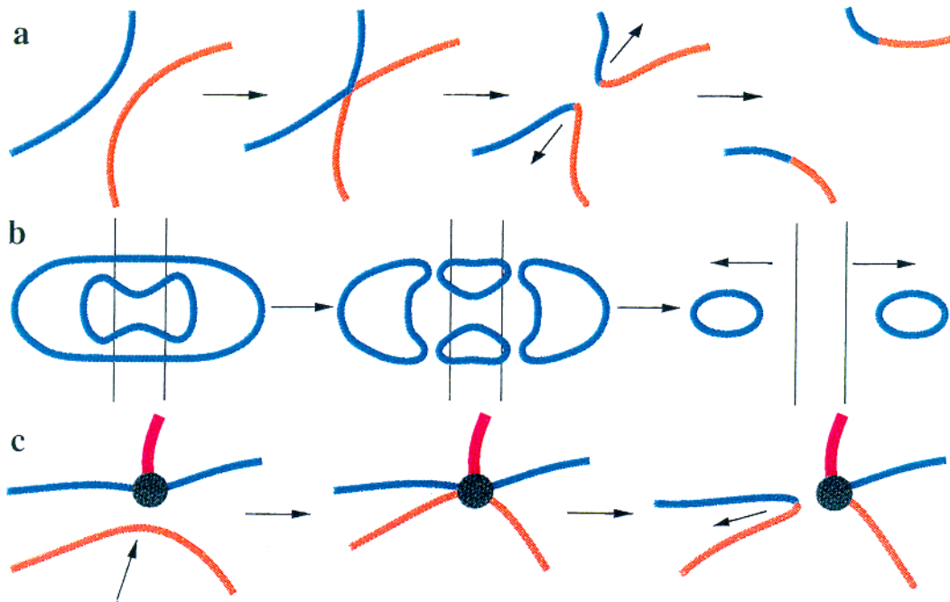
Fig. 24. Interaction of defect lines in the turbulent regime: (a) reconnection of lines following contact, (b) formation of bubbles disconnected from the shock line (indicated by two vertical solid lines), and (c) reconnection of lines in the wave core (indicated by black disk). The arrows between the pictures show the sequence of events, while arrows on the pictures designate the direction of line-defect motion.
