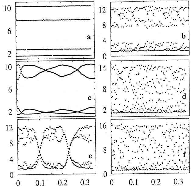
Fig. 20. Time series of the c_z concentration maxima: (a and b) C = 4.30 , (c and d) C = 4.42 and (e and f) C = 4.7 . Left panels show the local dynamics at a point in the bulk, while the right panels show the dynamics on the shock lines. Time is in units of thousands of spiral revolutions. In panels (c) and (e), respectively, the crossing of the c_z maxima reflect the passages of an \Omega_2 or \Omega_1 line through the observation point in the medium.
