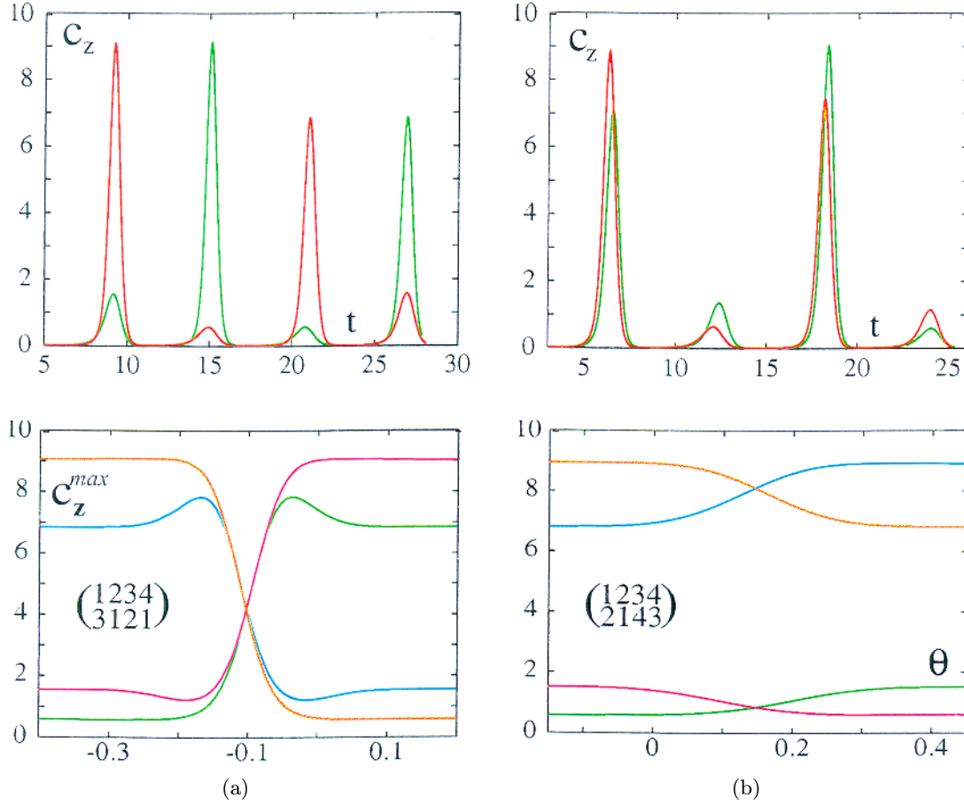
Fig. 13. Structure of synchronization defect lines in the period-4 regime: (a) \Omega_1 defect, (b) \Omega_2 . Upper row of panels shows local c_z(t) time series calculated on the opposite sides of corresponding defect lines. Lower row of panels displays corresponding loop exchanges (see text). Lines of the same color correspond to c_z(\theta) maxima calculated at the same time instant.
