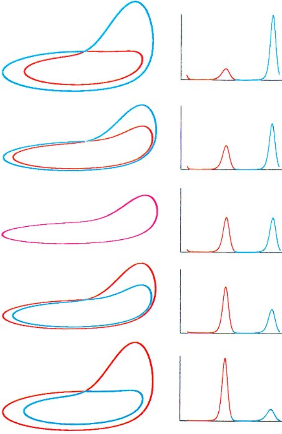
Fig. 8. Loop exchange in local orbits as the \Omega curve is crossed. Right column displays the c_z(\theta, t) time series corresponding to the orbits in (c_x, c_y, c_z) phase space shown in the left column. To highlight the exchange the first half of an oscillation period for each orbit is colored differently from the second half.
