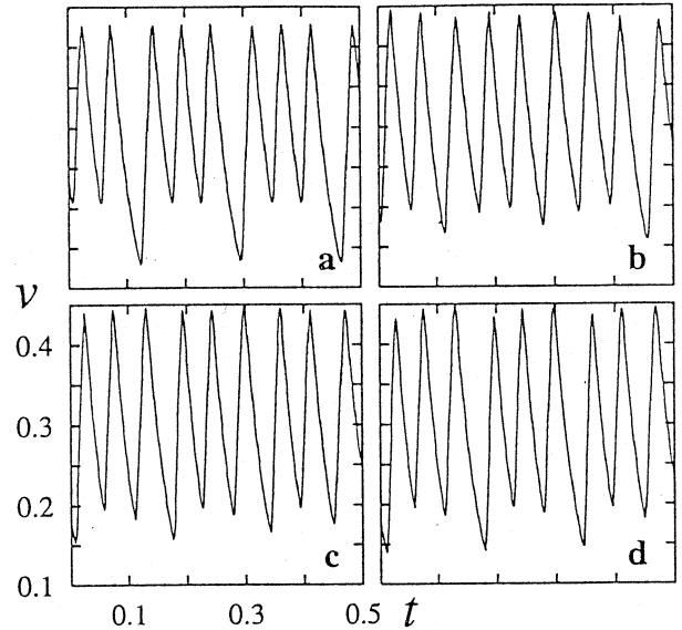
Fig. 9. Change in character of local dynamics across one of the defect lines seen in Fig. 5. See text for details.
