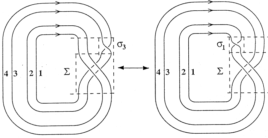
Fig. 26. Two alternative configurations of the \overline{B}_4 braid: \Sigma_1 = \sigma_3 \Sigma (left) and \Sigma_2 = \sigma_1 \Sigma (right).
