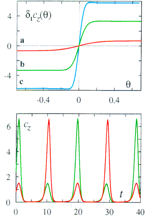
Fig. 7. The change of the local dynamics across the \Omega curve. Upper panel shows \delta_1 c_z(\theta) along the arc at radius r_0 = 130 indicated in Fig. 4 for three values of C : (a) C = 3.04 , (b) C = 3.10 , (c) C = 3.84 . Bottom: two c_z(t) concentration time series calculated at points \mathbf{r}_{1,3} = (r_0 = 130, \theta_\Omega \pm 0.05) on opposite sides of the \Omega curve.
