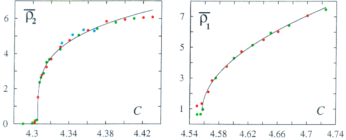
Fig. 21. Transition to (left) \Omega_2 - and (right) \Omega_1 -line turbulence. (Green) System with two spirals shown in Fig. 19; (red) system of the same size with four spirals; (blue) system with two spirals but twice the linear dimension, L = 512 .
