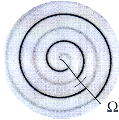
Fig. 4. Spiral wave in the Rössler medium with no-flux boundary conditions and period-2 local dynamics at C = 3.84 . Concentration field c_z(\mathbf{r}, t) is shown as gray shades. The solid line depicts the \Omega curve. Dynamics on the small arc segment that transversally cuts the \Omega curve will be described below.
