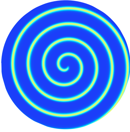
Fig. 1. A spiral wave in a disk-shaped oscillatory medium with no-flux boundary conditions and dynamics described by the Rössler reaction-diffusion equation in the period-1 regime. The c_z(\mathbf{r}, t) concentration field at a single time instant is displayed.
