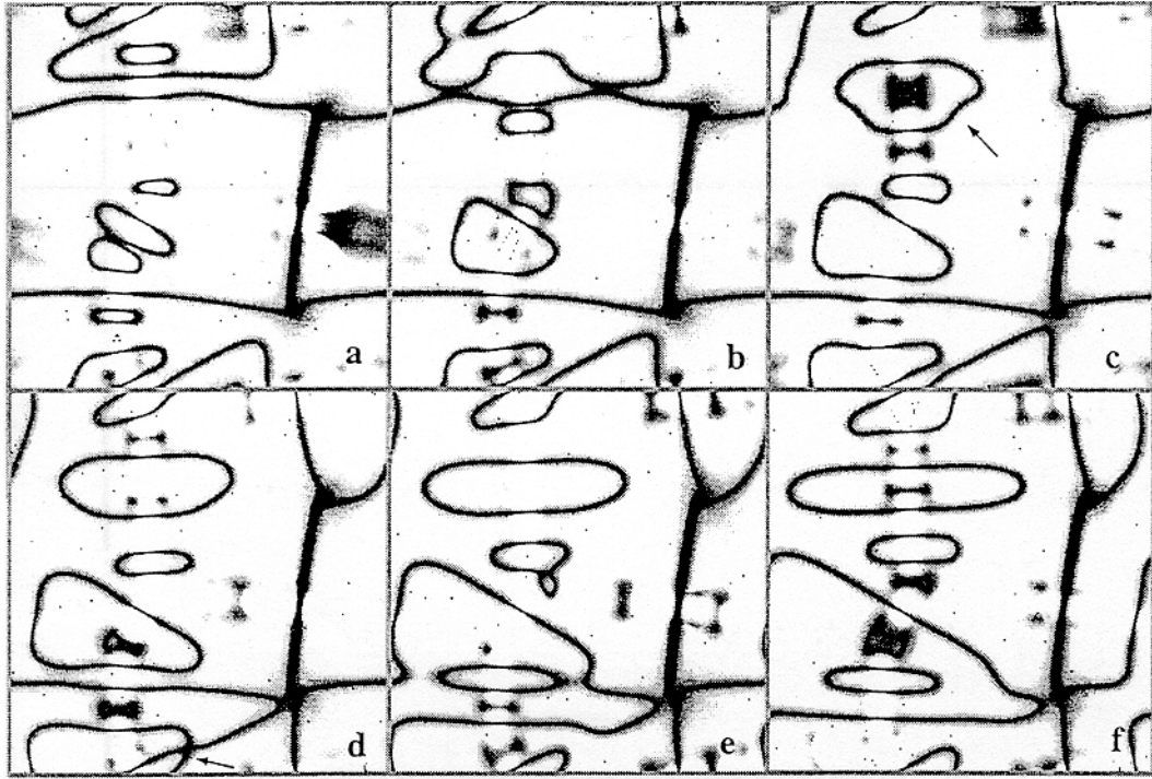
Fig. 23. The evolution of the medium with \Omega_2 -line turbulence at C = 4.38 . All panels are equally separated in time by 24 spiral revolutions and show the \xi_2(\mathbf{r}) field coded by gray shades.
