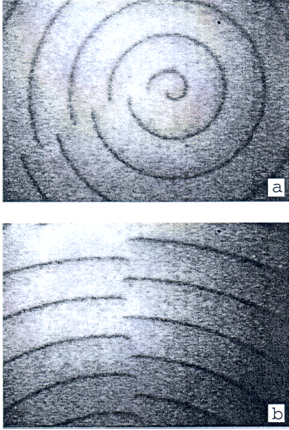
Fig. 6. Spiral wave with synchronization defect line on the surface of the ruthenium catalyzed BZ reagent. Panel (b) shows continuation of the defect line seen in panel (a). Reproduced with permission from [Yoneyama et al. , 1995].
