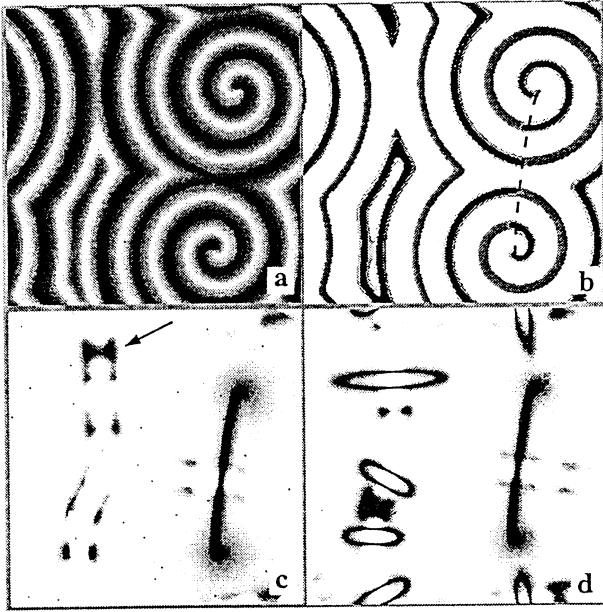
Fig. 19. Representation of defect lines by the \xi_2(\mathbf{r}) field for the medium with two spiral waves at (c) C = 4.30 and (d) C = 4.32 . Panels (a) and (b) show, respectively, the \varphi(\mathbf{r}, t_0) and c_z(\mathbf{r}, t_0) fields calculated for the medium in panel (c).
