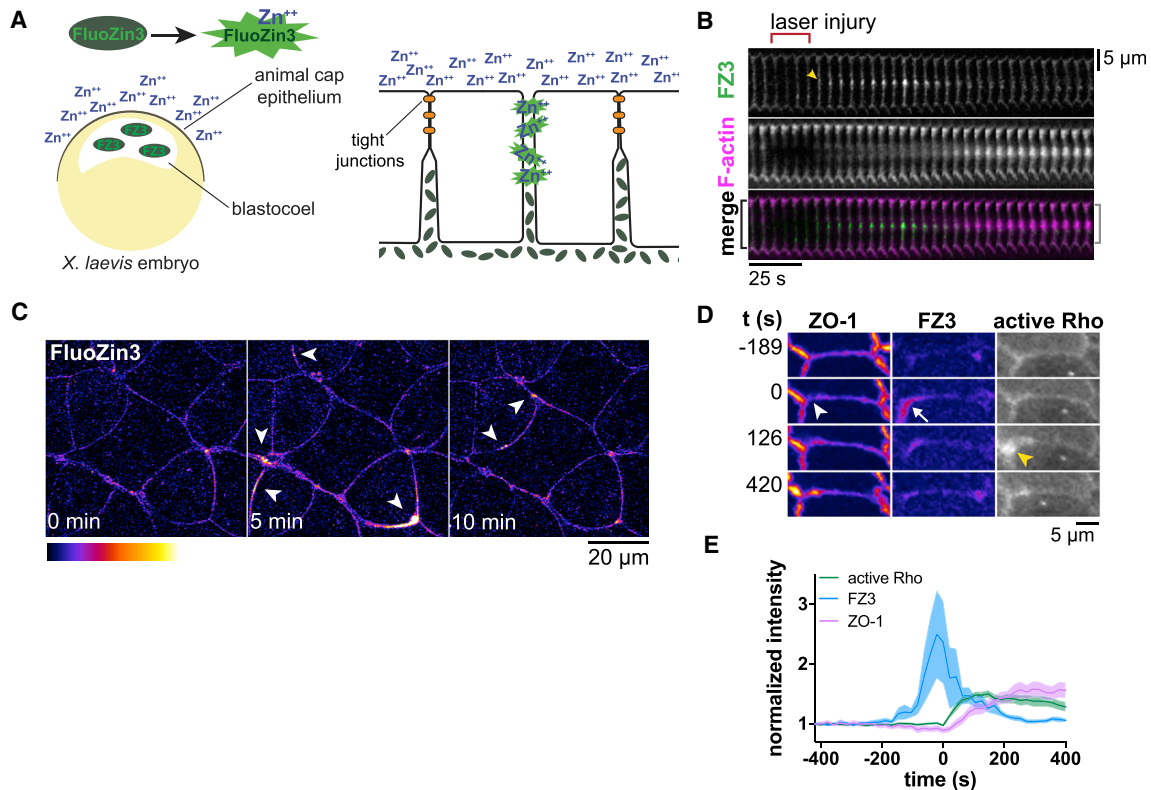
Figure 1. Transient, Localized Leaks in the Tight Junction Barrier Are Followed by Flares of Active Rho and Restoration of Barrier Function (A) Schematic of Zinc-based Ultrasensitive Microscopic Barrier Assay (ZnUMBA). Exchange of zinc and FluoZin-3 (FZ3) through disrupted tight junctions yields a local increase in FZ3 fluorescence. (B) Validation of ZnUMBA by laser injury of the junction (red bracket). FZ3 (green) increases in intensity (yellow arrowhead) following laser injury and persists for roughly 75 s. Note that F-actin (Lifeact-RFP, magenta) accumulates at the site of injury, and the junction contracts (black bracket versus gray bracket). (C) FIRE Lookup Table (LUT) applied to FZ3 in the unperturbed Xenopus laevis epithelium. Arrowheads indicate short-lived, localized barrier leaks. (D) Leaks (FZ3, white arrow) occur at sites of local ZO-1 loss (white arrowhead), and Rho flares (yellow arrowhead) follow at these sites. FZ3 intensity decreases while ZO-1 intensity increases following Rho flares. (E) Mean normalized intensity for active Rho (mCherry-2xrGBD), FZ3, and ZO-1 (BFP-ZO-1) at the site of the Rho flare over time quantified from (D) and additional videos. Shading represents standard error of the mean (SEM). n = 17, 7, and 5 (flares, embryos, experiments, respectively). See also Figure S1 and Videos S1, S2, and S3 .
